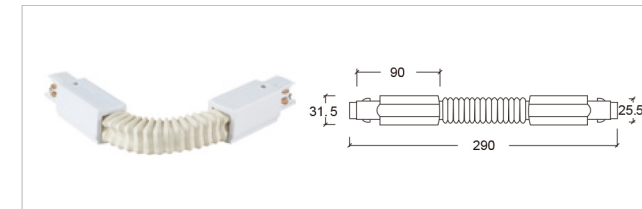
Flexible Connector
