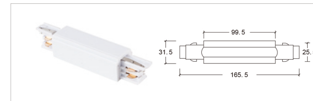
Straight connector
