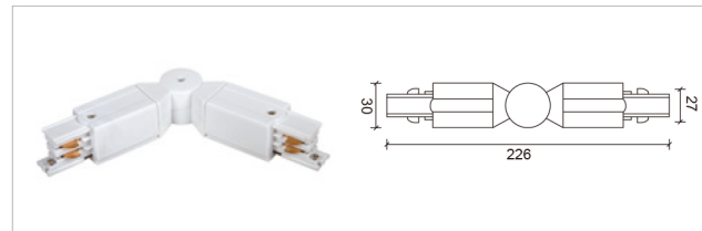
Flexible Connector
