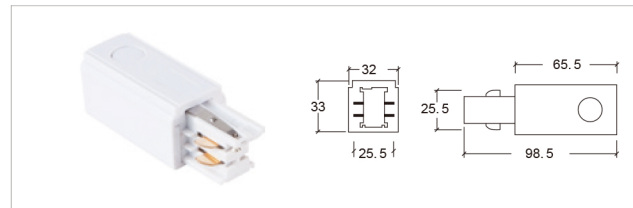
Feeder-L
