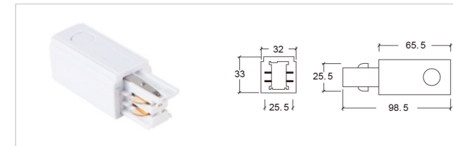
Feeder-R
