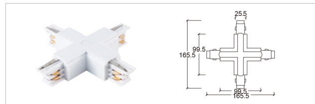
X- connector
